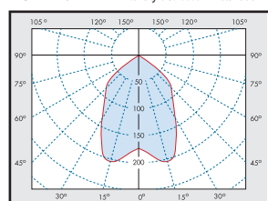
ASM 226 Intensity distribution in cd/1000lm
