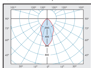
ASM 70 Intensity distribution in cd/1000lm
