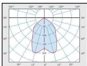
ASR 226 DM Intensity distribution in cd/1000lm
